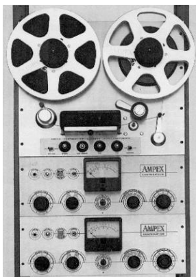
Fig. 9. Two-Channel Model 350, Rack Mounted
