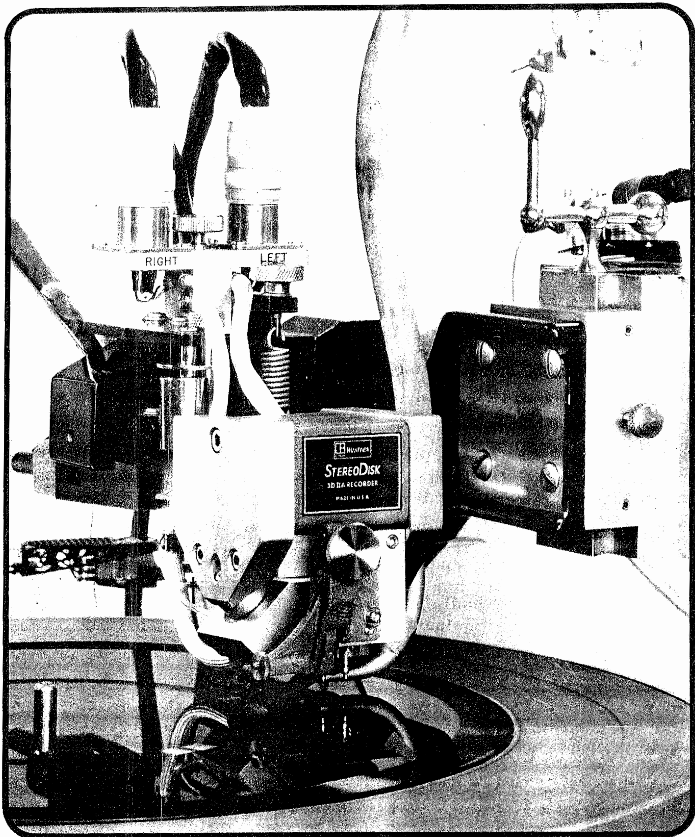
The Wextrex 3DII AH Stereo Cutterhead. (Manufacturer's photo)
