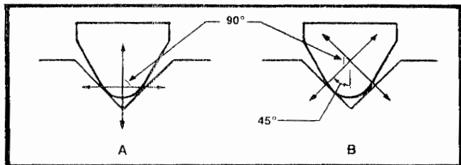
Technique A is the obvious way to cut two channels in a single groove. This method is extremely difficult.
