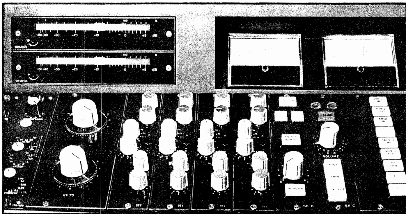
Both peak and VU metering are handy in disc cutting.
