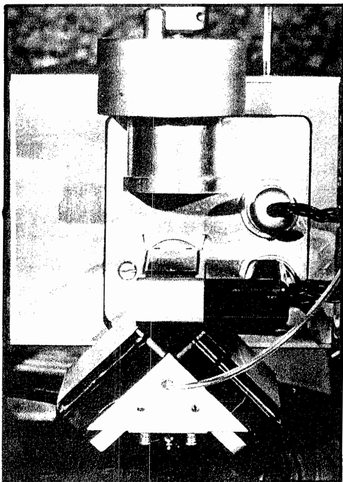
The Neumann SX-74 Stereo Cutterhead.
