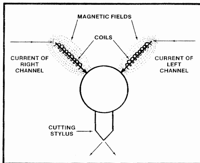
Simplified view of a stereo cutterhead.
