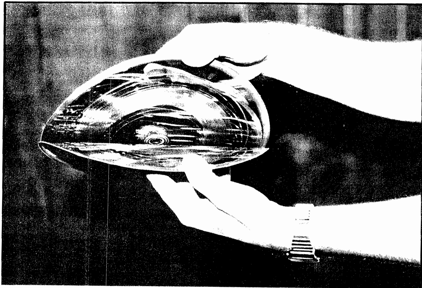
Separating the metal master and the mother.
