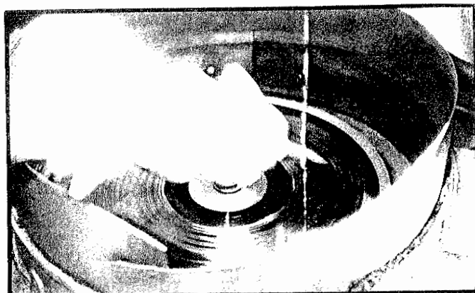
Polishing a metal mother helps get rid of "horns".
