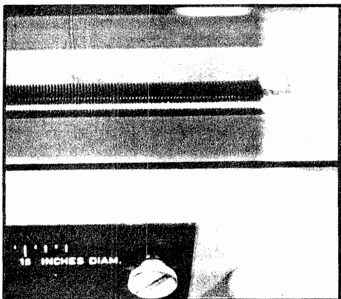
The lead screw of a Neumann Lathe. The carriage rides on this screw on its journey across the disc. The "pitch" is changed by speeding up or slowing down the motor which turns it.
