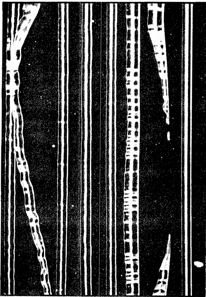
Overcuts, lift-outs and proper groove depth can be seen through the microscope.
