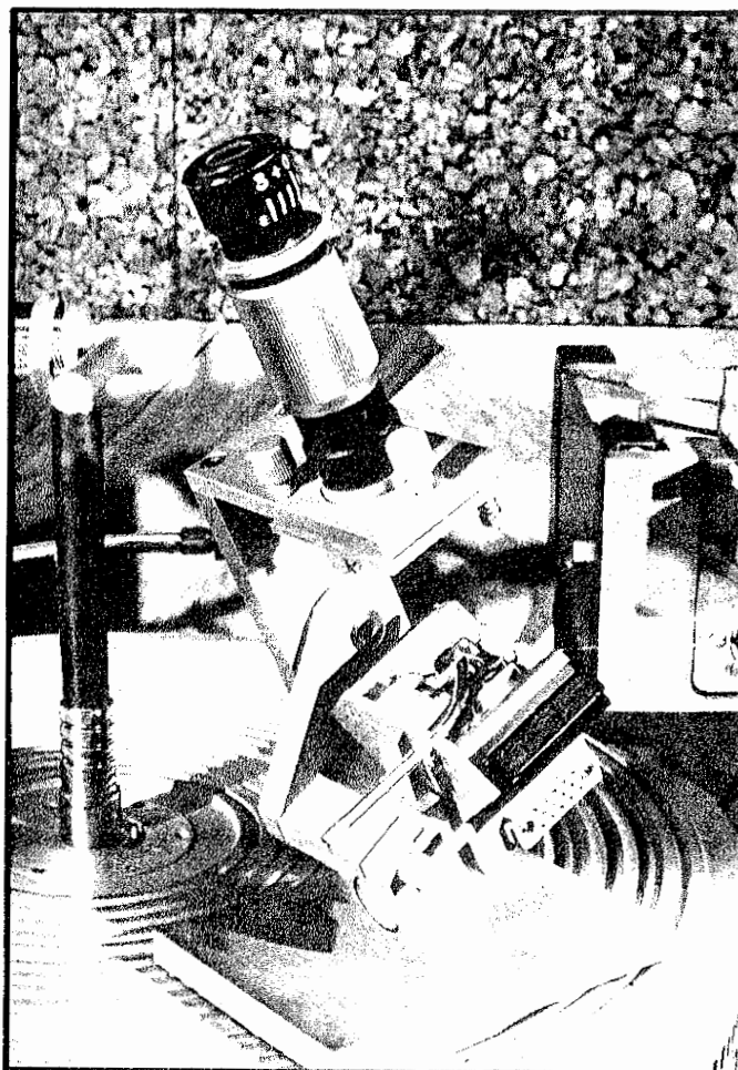
A second, smaller microscope is used to mount the cutting stylus in the cutterhead.
