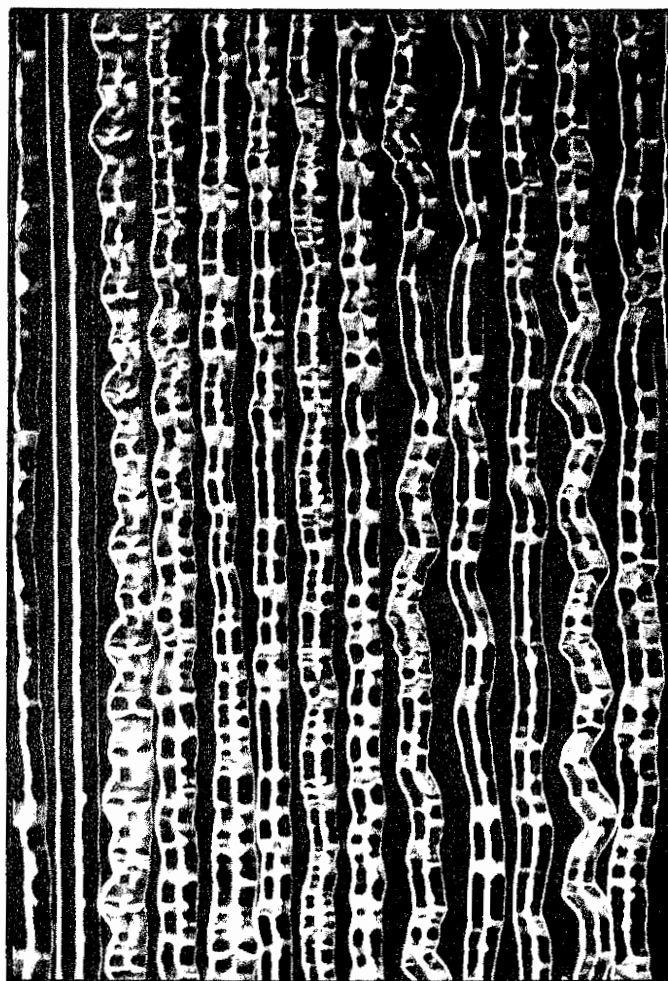
Variable pitch at work, controlling groove spacing to avoid overcut.
