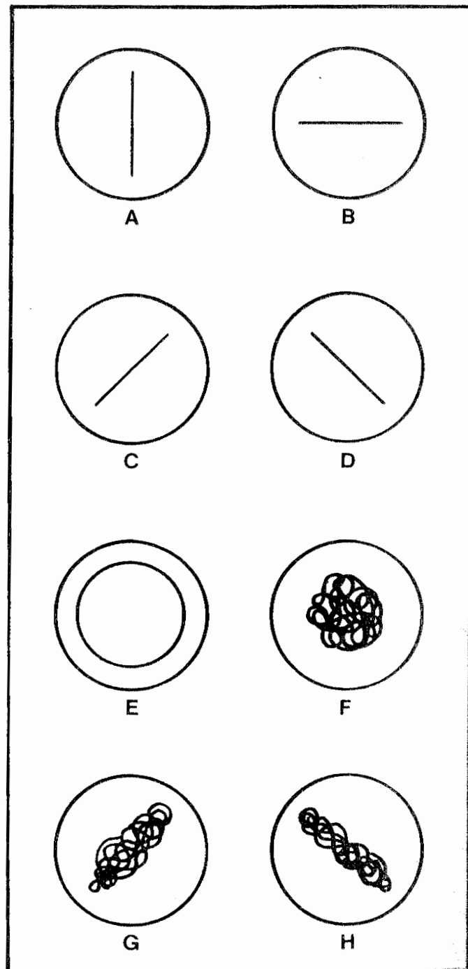
Common oscilloscope patterns. A. Left channel only; B. Right channel only; C. Stereo, a combination of A and B; D. Stereo as C, but 180° out of phase; E. Phase shift of 90°, seen when aligning azimuth of playback tape machine; F. Random stereo, such as might be seen on a multi-miked recording. Some out of phase material present; G. Stereo program which is largely in phase; H. Stereo program which is largely out of phase.
