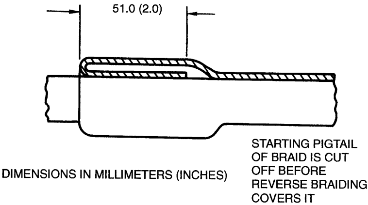
Figure 9-8. Starting Lock
