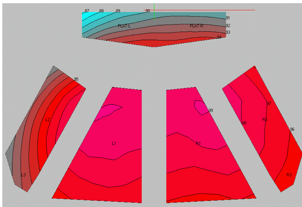
Fig 7. Predicted direct sound for a loudspeaker delayed by 18 ms added to the left channel loudspeaker of Fig. 6. Contours of equal level are at 1 dB increments. The delayed loudspeaker is 1.5 m to the left of centerline, is aimed to the right rear corner of the audience, and is operating at 3 dB below the level of the main left loudspeaker.
