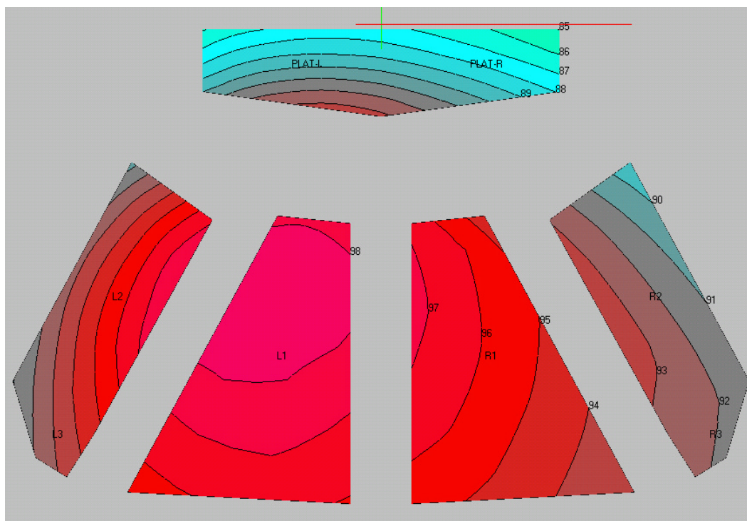
Fig 6. Predicted direct sound from a single 90°x 40° loudspeaker, 9 m left of center, aimed to the center rear of the right center seating in the room of Figs. 4 and 5.
