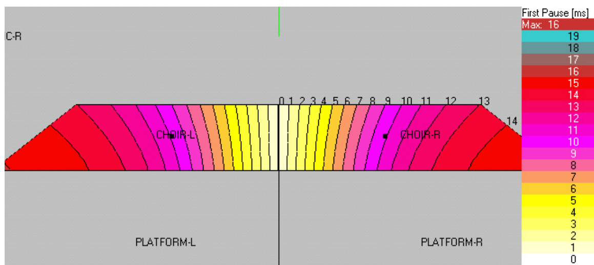
Fig. 10 Predicted arrival time differences (ms) for singers at various locations throughout a choir for a pair of microphones spaced 5.5 m apart and suspended 2.5 m above and 2 m downstage of the choir. As compared to a singer on centerline, a singer 3 m to the left of center is about 6 ms closer to the left microphone and 4 ms farther from the right microphone. These differences add (algebraically) to the travel time differences between the loudspeakers and the listener, and strengthen the stereo image for off-center sources and listeners.
