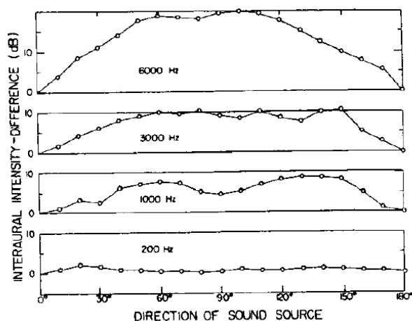
Fig. 1 Interaural intensity difference measured at the two ears as a function of the azimuth of the sound source [14] Reference 15 includes more detailed data.
