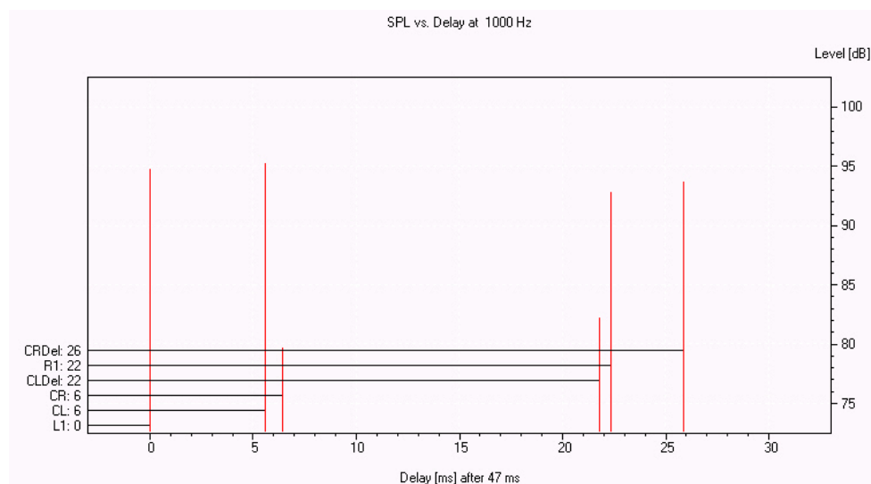
Fig 9 EASE prediction of direct sound arrivals at a seat near the left rear corner of the left center seating bank. A study of the results of calculations like this one is required for seats throughout the audience to verify that the design meets the criteria for good stereo.
