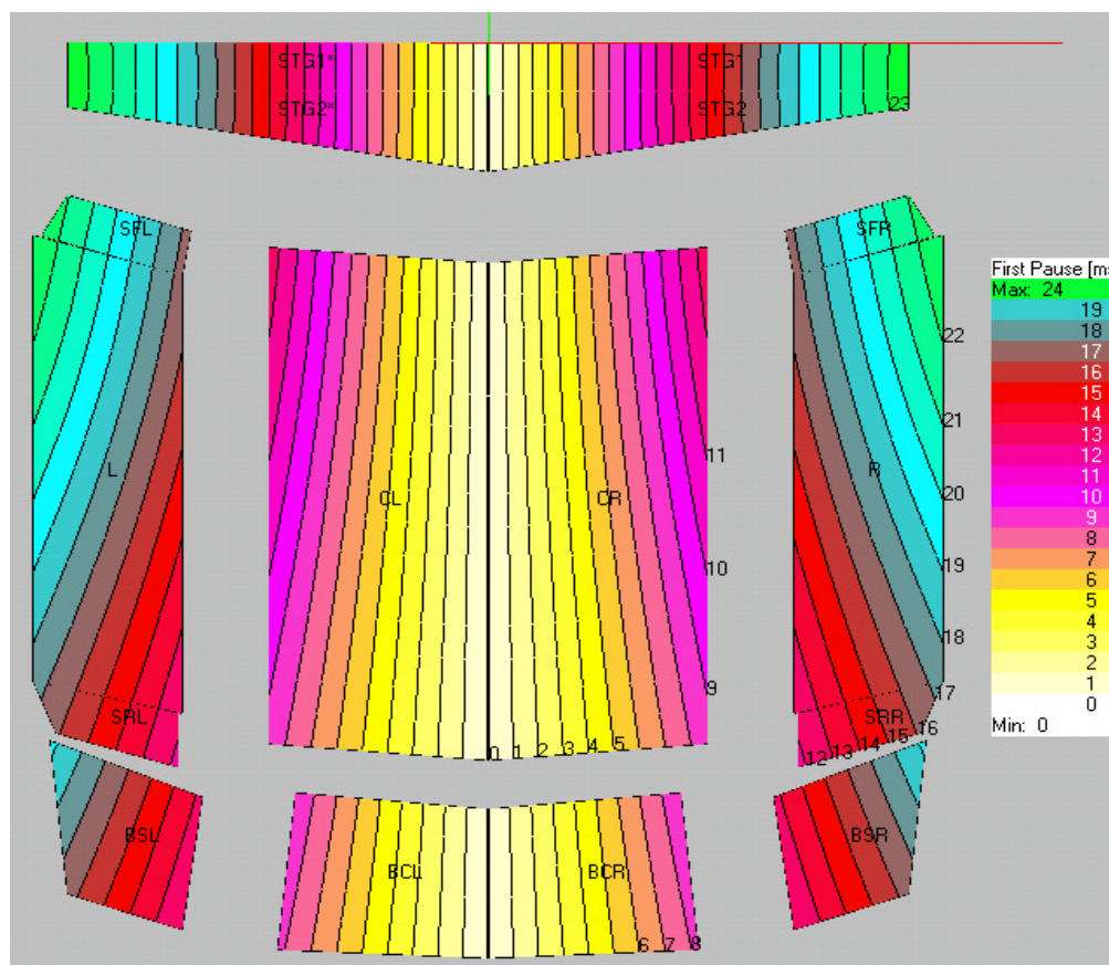
Fig 3. The EASE prediction of the difference in arrival times for left and right channels for a simple stereo system in a small theater. The greatest differences in arrival times occur at the front corners of the audience, the smallest differences are at the rear of the audience. Contours are at 1 ms increments.
