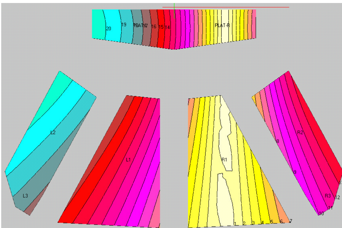
Fig 5. Predicted arrival time differences for right and center front clusters in the same room and at the same height as Fig 4. Contours of equal delay are at 1 ms increments, and the criteria for arrival times is met in all seats.
