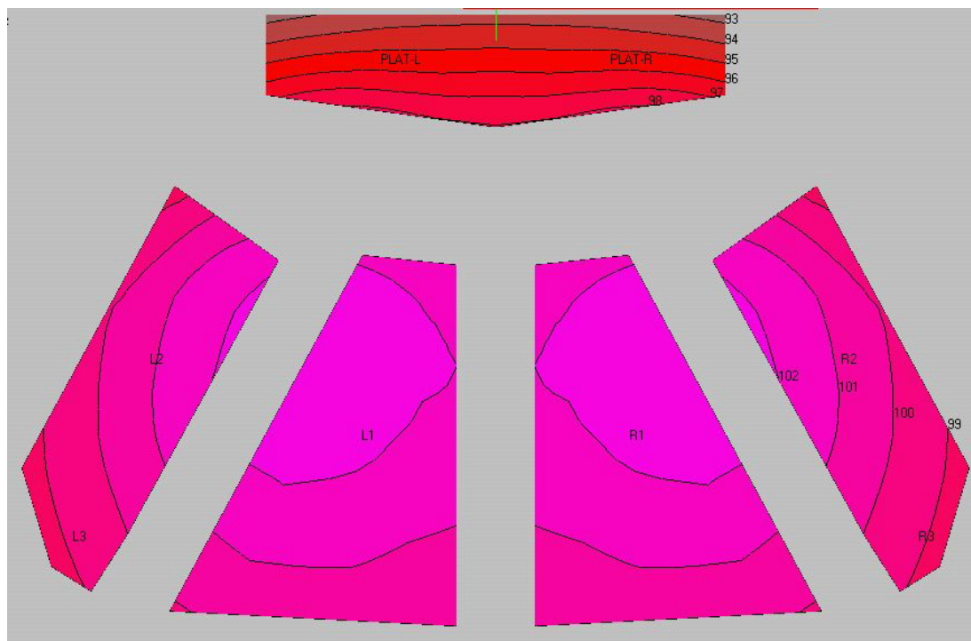
Fig 8. Predicted direct sound for all three channels, including delayed loudspeakers. Contours of equal level are 1 dB increments.
