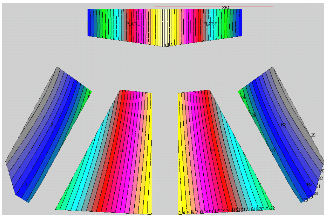
Fig 4. Predicted arrival time differences for left and right front clusters in a wide room with a relatively low ceiling (9 m above the stage). Contours of equal delay are at 1 ms increments, and the criteria for arrival times is not satisfied in much of the side seating areas.
