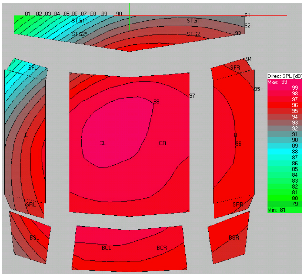
Fig. 4. The EASE prediction of direct sound for the left channel only. Contours are at 1 dB increments. The five sided audience area at the top of the plot is the forestage.
